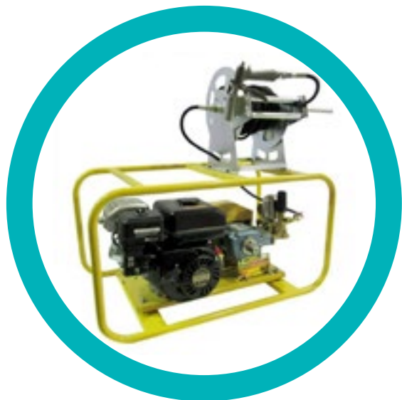
Rato Semi Fire Fighter (No Tank)
