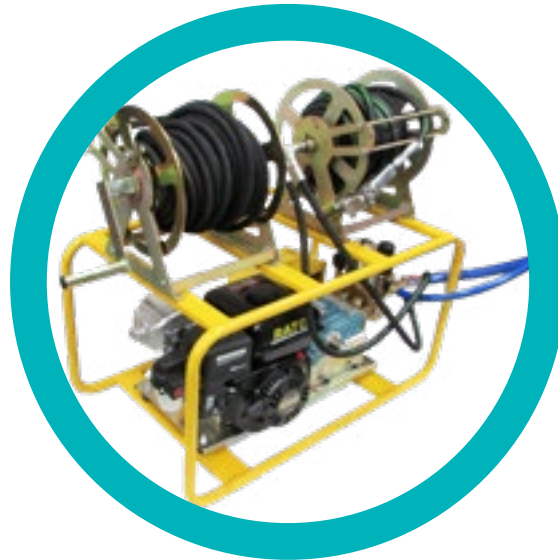
Rato Double Reel Semi Fire Fighter (No tank)
